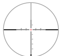
4-16X44 / SFP ETCHED GLASS UMOA / IE® 36-COLOR / OP3-GM4164UMOA
